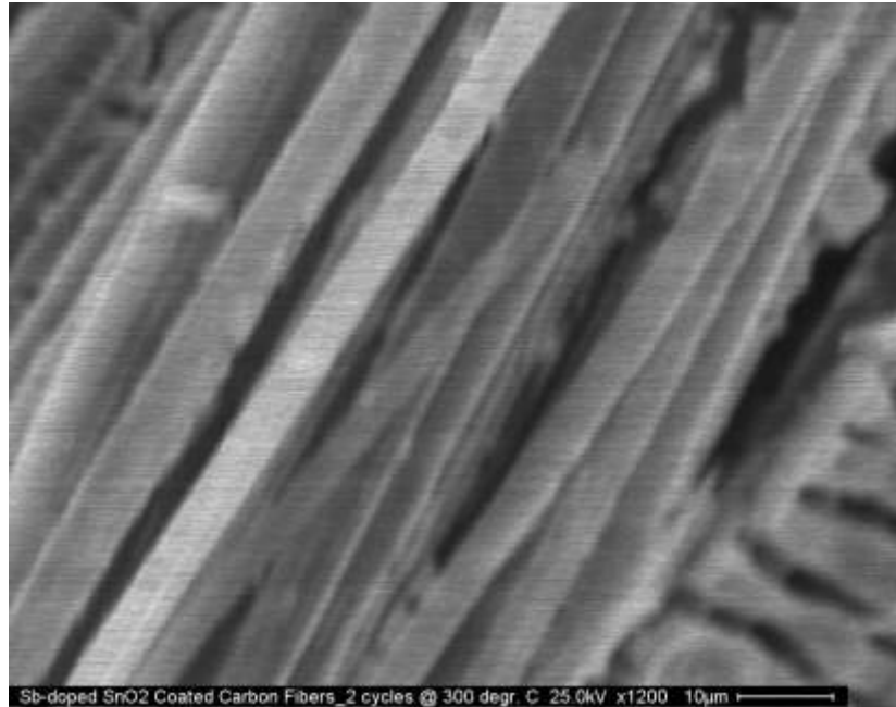
Figure 5.3.2. ATO coated carbon fibers heat treated at 300 °C.
