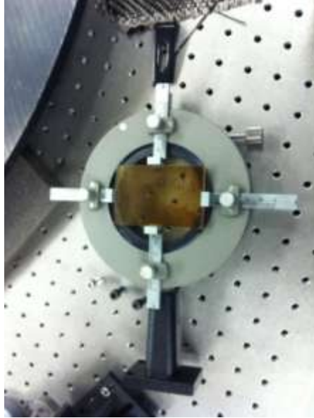
Figure 6.2.3. ATO( \text{Co}_2\text{O}_3 ) sol-gel coated quartz slide in the optics sample holder for bi-static angular-dependent transmittance measurements.
