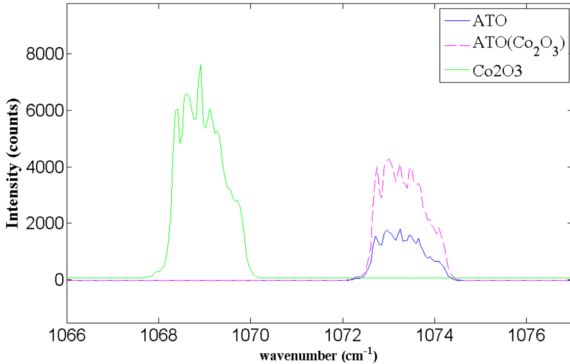
Figure 4.5.4. Raman spectroscopy of ATO(Co 2 O 3 ) after one cycle of spin coating/heat treatment at 200 °C.[88]
